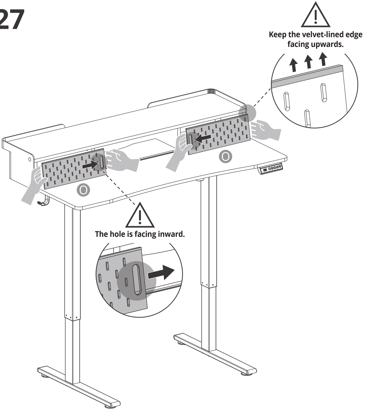
1 Angled Insertion
